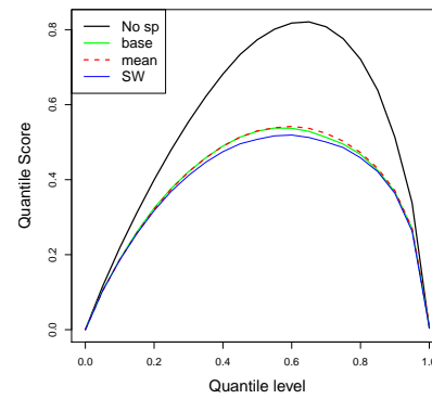
Figure 5.20: Comparison of the Brier Score plots and quantile decomposition plots obtained with the different model specifications on all the hours and events pooled together.
