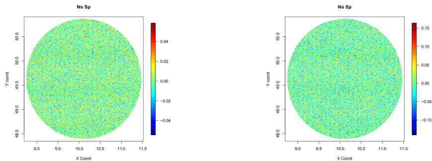
Figure 5.15: Spatial effect for rainfall amounts obtained with Models “No Sp” on 19/09/2010 at 01 a.m. and on 18/09/2010 at 5 p.m.: mean of the posterior predictive distribution of \alpha .
