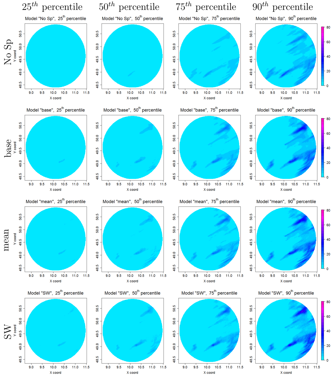
Figure 5.30: Map of the 25 th , 50 th , 75 th and 90 th predictive percentile with the four model specifications on 18/09/2010 at 05 p.m.
