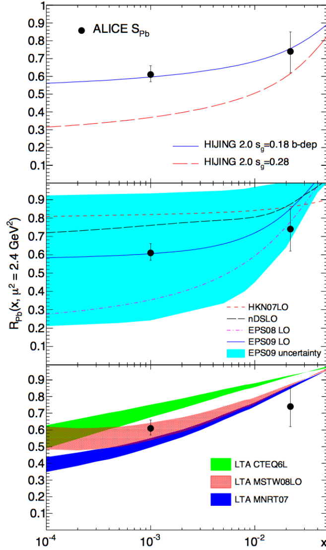
Figure 4.15 Comparison of the ALICE suppression factors with predictions of the nuclear gluon shadowing in HIJING 2.0 ( top ), global QCD fits ( middle ), and in the leading twist approximation ( bottom ) as computed by [22].
