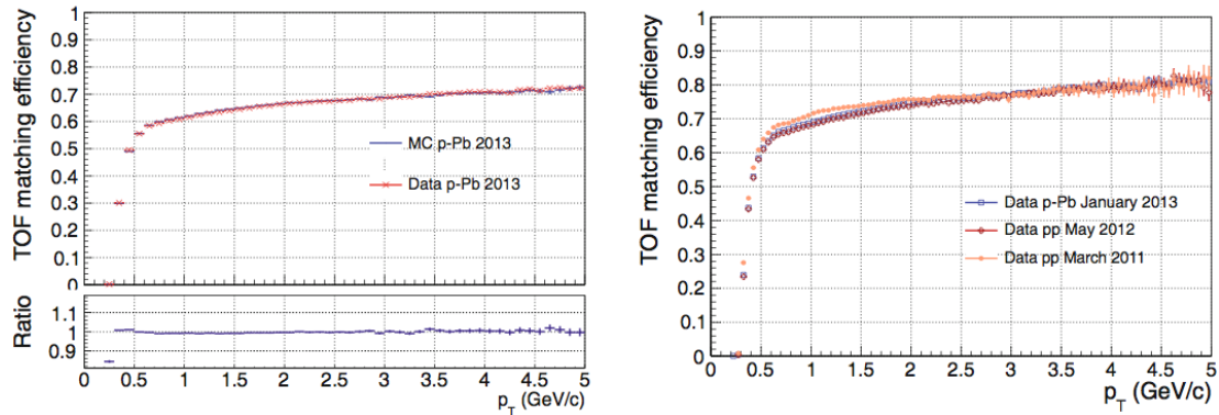
Figure 3.12 Left: comparison between the TOF matching efficiency measured in 2013 p - Pb data and the one extracted from the corresponding simulation ( top ) and their ratio ( bottom ). Right: comparison between the TOF matching efficiency measured with 2011, 2012 p - p data and with 2013 p - Pb data, as in [89].
