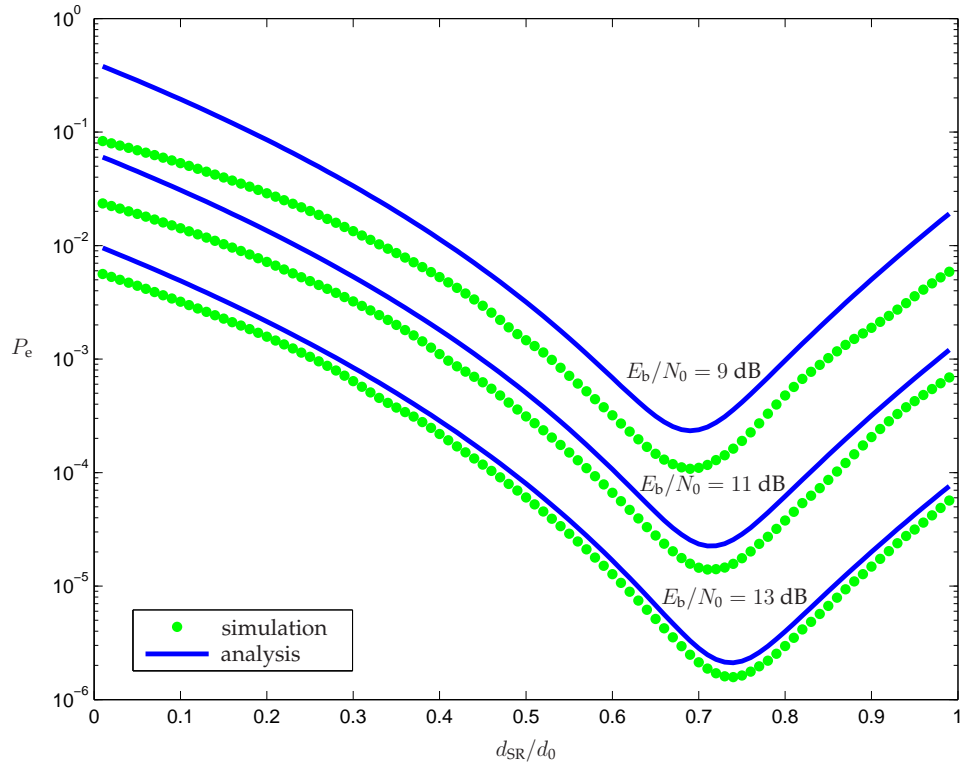
Figure 2.8: P-STCs case study: P_e as a function of d_{\text{SR}}/d_0 for different values of E_b/N_0 (dB); comparison between (2.6) and simulations.
