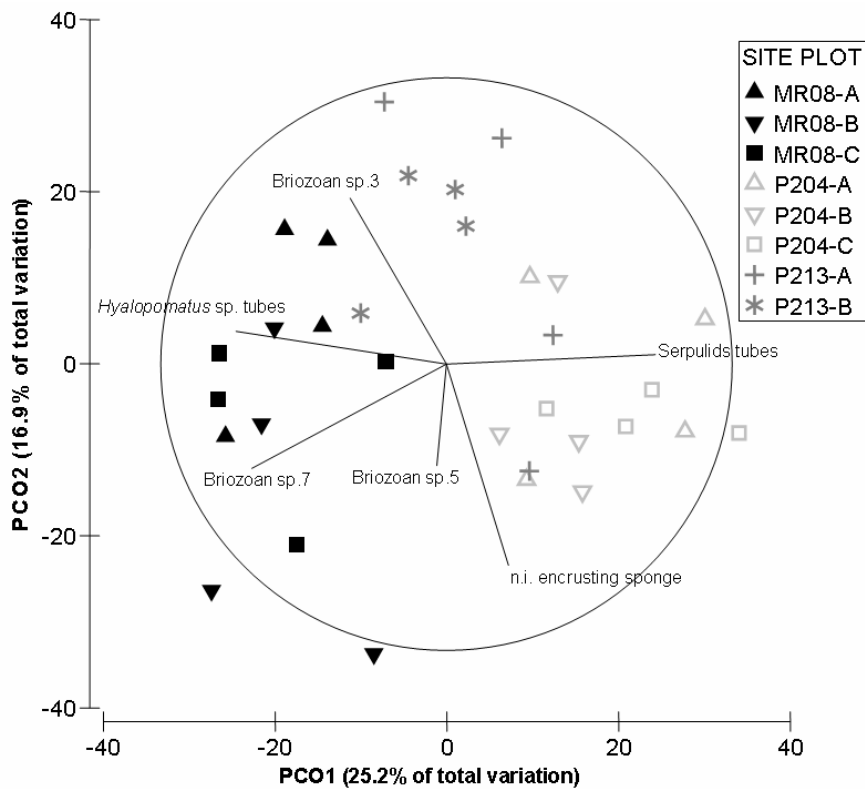
Figure 2. PCO unconstrained ordination plot (i.e. metric MDS) based on Bray-Curtis similarities of square root-transformed percent cover data, the superimposed vectors represented correlation of single taxa with PCO Axes: a) percent cover of sessile organisms colonising the upper face b) percent cover of sessile organisms colonising the lower face.
