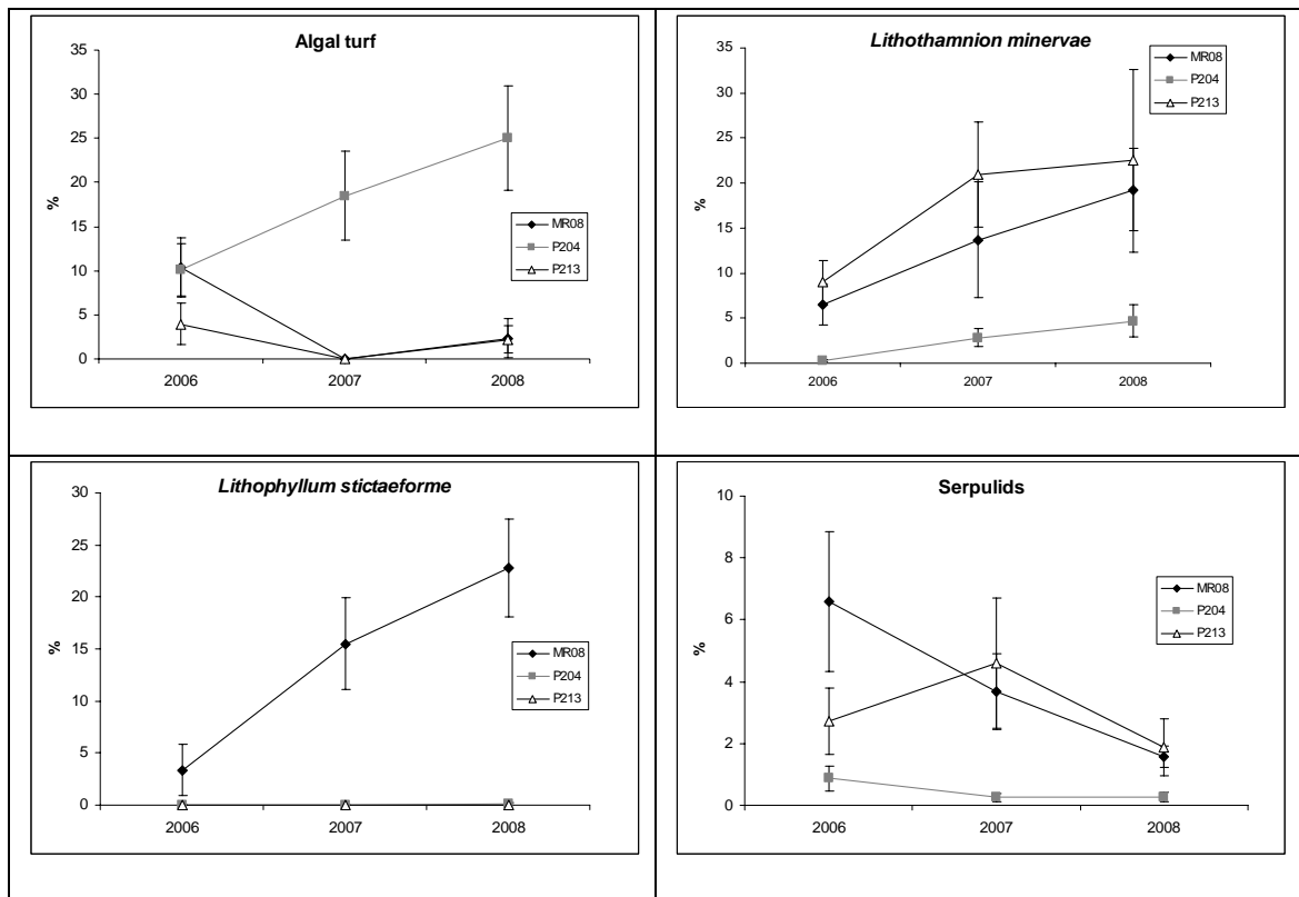
Figure 6. Spatial and temporal trends of the selected species: a) Algal turf b) Lithothamnion minervae , c) Lithophyllum stictaeforme , d) serpulid polychaetes (mean values ± SE).
