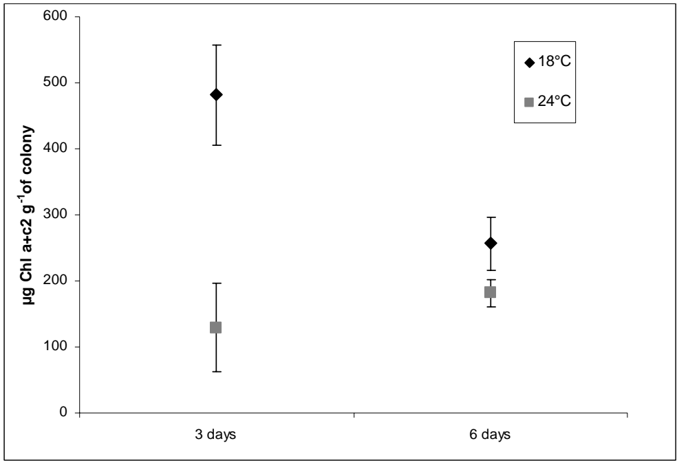
Figure 1 Concentration of chlorophyll a + c2 in relation to the exposed temperature.
