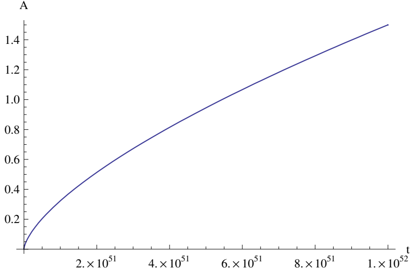
Figure 3.1.: Plot of the ratio \mathbf{A} for the model I , with the parameter choice \alpha = 1(t_P/m_P)^{1/2} , k = 10^{-55}t_P^{-1} . It can be easily seen that at a time scale of order 10^{51}t_P the ratio becomes greater than 1.
