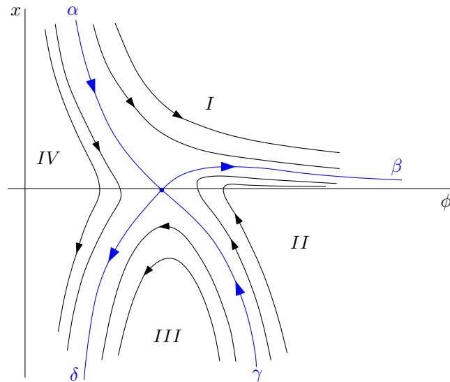
Figure 5.2.: Positive \phi -axis phase portrait for the dynamical system (5.11) with h \geq 0 . The four separatrices of the saddle point (\alpha, \beta, \gamma, \delta) individuate four regions (I, II, III, IV) with different behaviors of the trajectories, as explained in the text.
