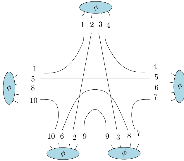
Figure 8.7.: Interaction term of the 4d GFT model (8.92).
