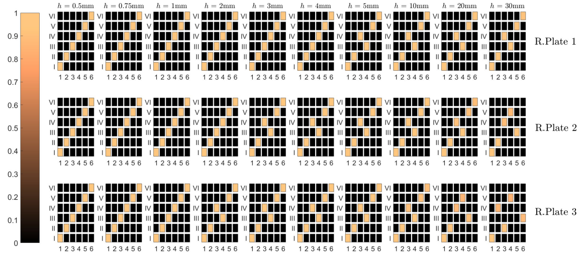
Fig. 5.3 MAC plots for rectangular plates (R.Plates) compared against the baseline configuration. Each column corresponds to a different plate thickness, while each row represents an increasing surface area: Plate 1 ( A = 1.92 \text{ m}^2 ), Plate 2 ( A = 0.48 \text{ m}^2 ), and Plate 3 ( A = 0.12 \text{ m}^2 ), from top to bottom.
