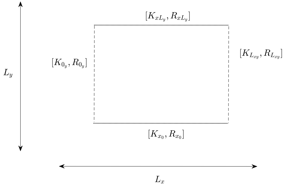
Fig. 4.24 Illustration of translational and rotational spring constants along plate edges
