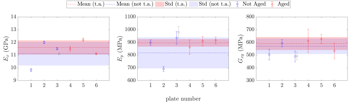
Fig. 3.15 Comparison of estimated values for the E_x , E_y and G_{xy} elastic constants for all the six tonewoods samples under study. In red are reported the values for the thermally aged (' t.a. ') plates. In blue are reported the values for the not thermally aged (' not t.a. ') plates.
