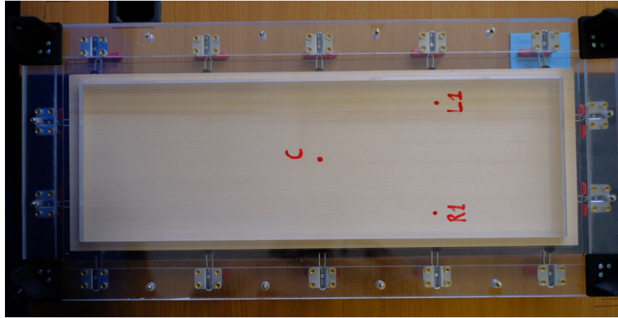
Fig. 4.1 Schematic representation of the measurement setup. The red dots L1 and C indicate the excitation points, namely locations for either the impact hammer hits or the contact point for the exciters while performing the validation measurements, while R1 indicates the position of the accelerometer.
