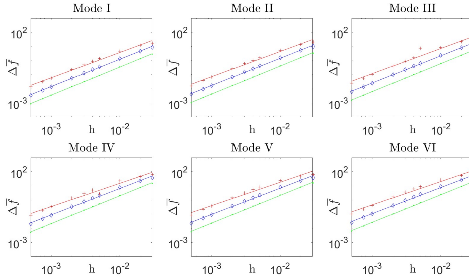
Fig. 5.6 Frequency deviations, computed using (5.5), as a function of thickness h for the six considered non-dimensional frequencies of the rectangular plates. Plate 3 ( A = 0.12 \text{ m}^2 ): red line with plus markers; Plate 2 ( A = 0.48 \text{ m}^2 ): blue line with diamond markers; Plate 1 ( A = 1.92 \text{ m}^2 ): green line with dot markers. For reference, a deviation of \Delta\tilde{f} = 100 corresponds to one semitone.
