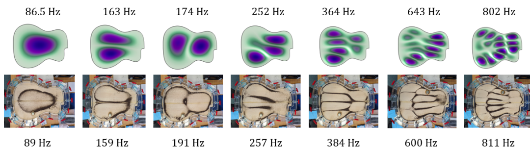
Fig. 4.28 Comparison between the modal behavior predicted by the FEM model of the guitar top plate and that observed experimentally through Chladni patterns on the physical board.
