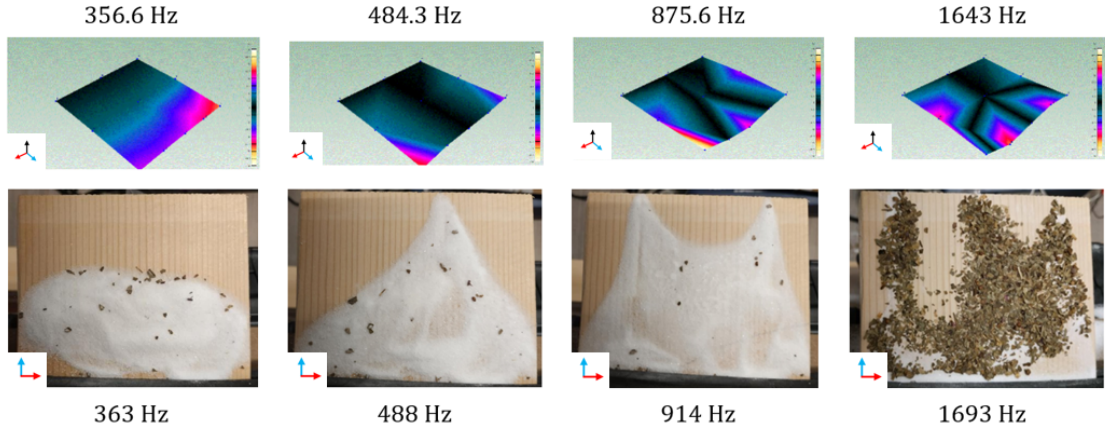
Fig. 4.19 Comparison of mode detection across the two experimental setups. Top row: identified experimental mode shapes. Bottom row: corresponding ODSs observed on the leftover plate sample.
