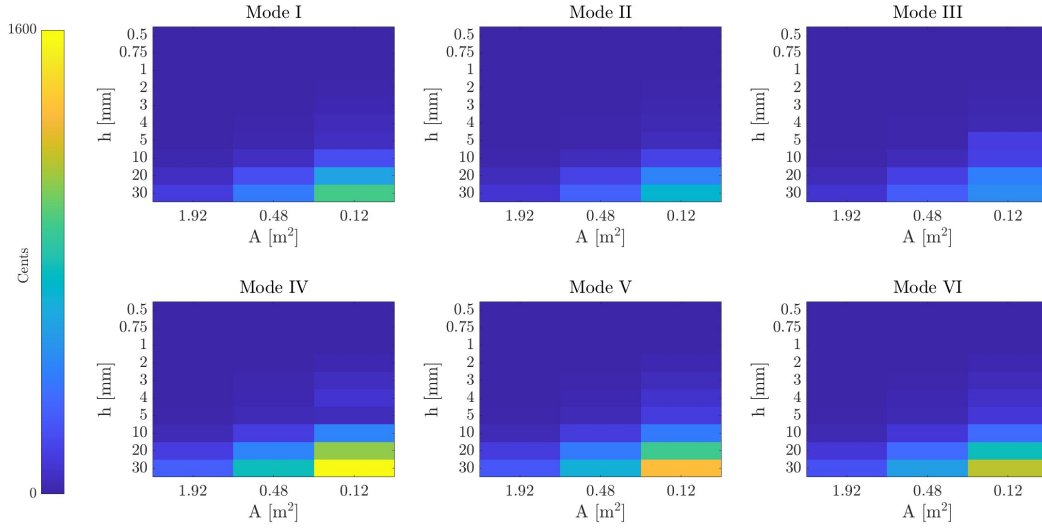
Fig. 5.5 Cent frequency deviations from the reference baseline (at h = 0.1 mm) for the rectangular plates.
