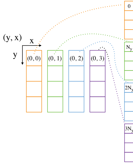
Figure 3.3: Arrangement of the finite difference plate as a linear vector.
