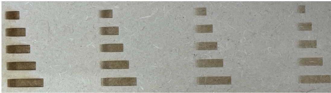
Figure 4.1: Test gradients of various heights using a laser cutter on MDF with decreasing laser power from left to right. The range of the gradient was too compressed to be differentiated by the optical sensor. On high power settings, scorching tends to bleed around the raster, thus affecting the surrounding material and area of the gradient.
