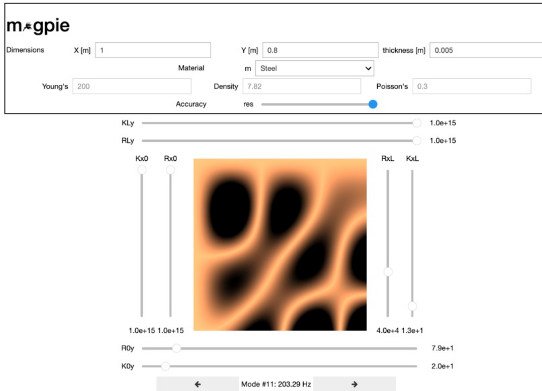
Figure 3.13: Beta version user interface for MAGPIE in Jupyter Notebooks.
