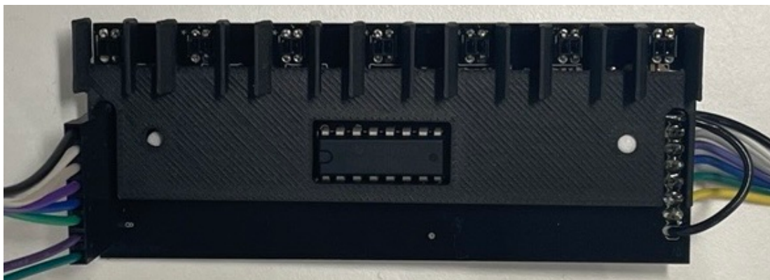
Figure 2.19: Sensor board front with baffles.
