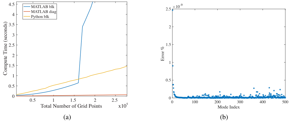
Figure 3.9: (a) Computational performance of the biharmonic assembled in a block format in MATLAB and Python and a diagonal format in MATLAB. Each size of biharmonic was computed 10 times and the shortest time was recorded. (b) Percentage error between MATLAB and SciPy for the first 500 eigenvalues.
