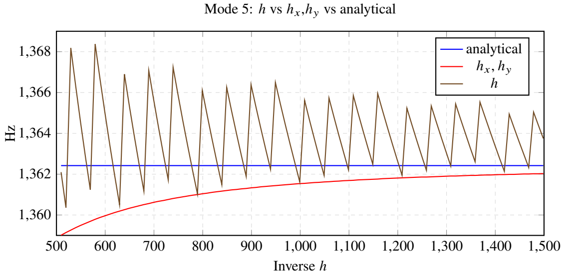
Figure 4.10: Comparison between analytic and modelled fifth mode of a plate for isotropic cases using shared and independent grid spacing in the x and y dimensions. Shared spacing shows saw-tooth convergence, while independent spacing converges smoothly.
