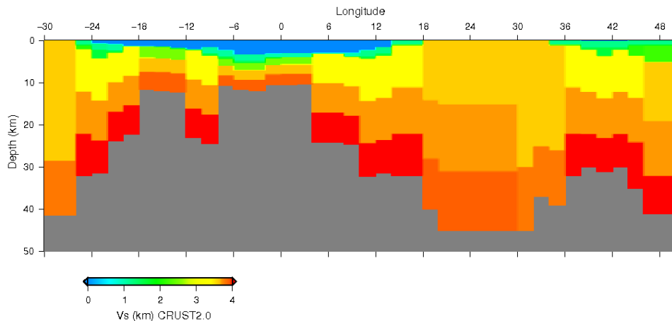
Figure 1.1: Vertical section of CRUST2.0 model. It's along the 70°N parallel and from -30^\circ\text{W} to 50^\circ\text{E} longitude.
