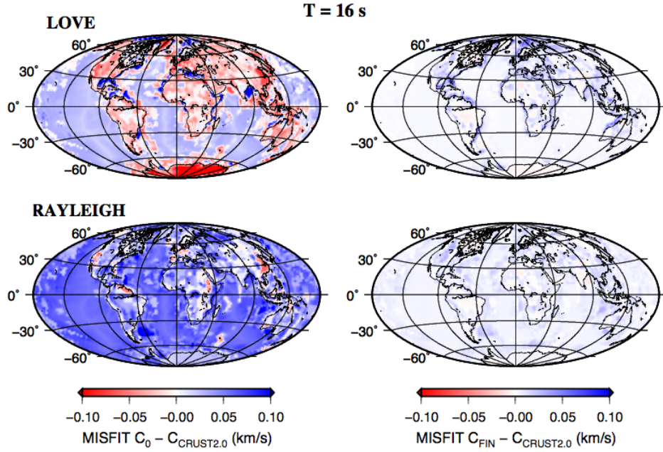
Figure 1.9: The same as in Figure (1.8) but for phase velocity at T=16\text{s} and for the CR-12KM model.
