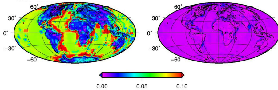
Figure 1.11: (left) RMS_d (1.5) between a-priori model and CRUST2.0 and (right) RMS_d between final 12KM model and CRUST2.0, after the inversion.
