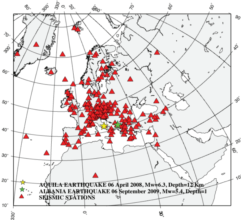
Figure 5.3: The map shows the station from ORFEUS network and the Aquila and Albania earthquakes selected for this study.
