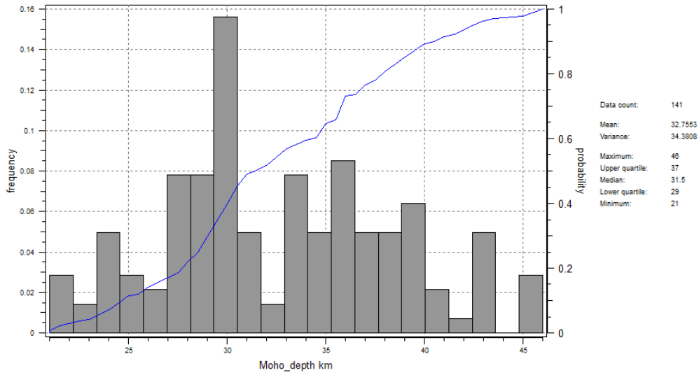
Figure A.1: Histogram for the Moho depth for the dataset used in Chapter 3
