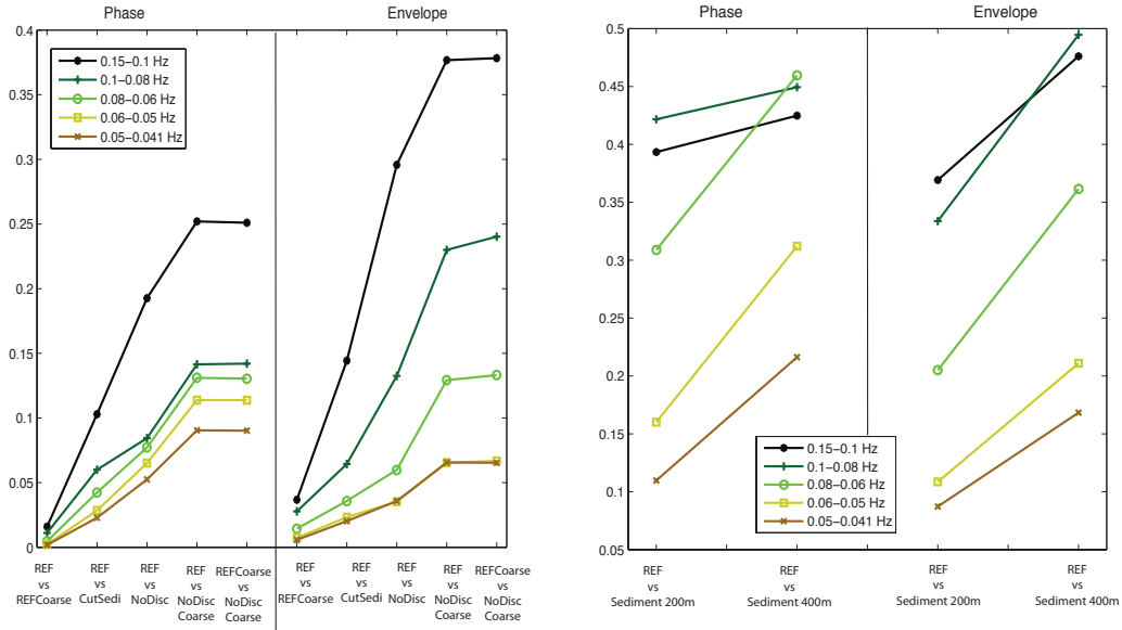
Figure 4.14: Cumulative misfit for the horizontal and vertical component for the sharp tests (left) and for the sediment interface deepening (right). Sum of the Envelope and Phase misfit of surface waves normalized by the number of the receiver times number of component (202). The colour lines are relative to different frequency range in which the misfit is calculated.
