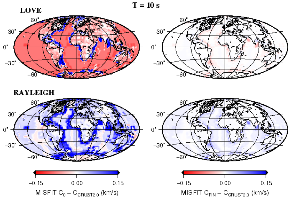
Figure 1.8: (left) Misfit between a-priori model and CRUST2.0 phase velocity at T=10 s for Love (top) and Rayleigh wave (bottom). (right) Misfit between CR-4KM final model and CRUST2.0 phase velocity at T=10 s for Love (top) and Rayleigh wave (bottom) for the whole Earth.
