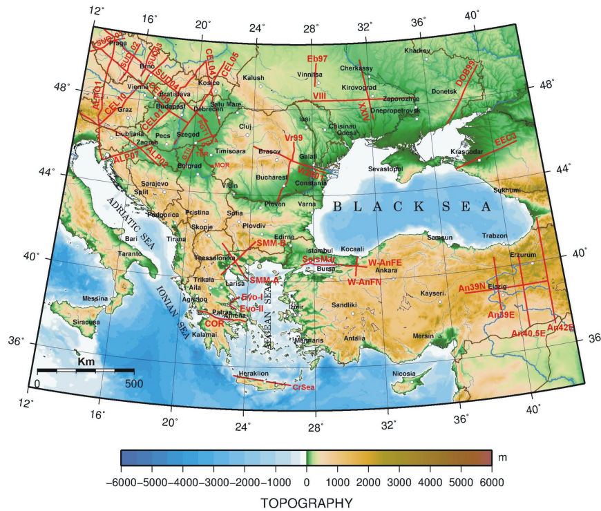
Figure 3.1: Location of the crustal seismic lines (red) used for testing of the EPCrust model on the background of the Geographic map of the Central and South East Europe.
