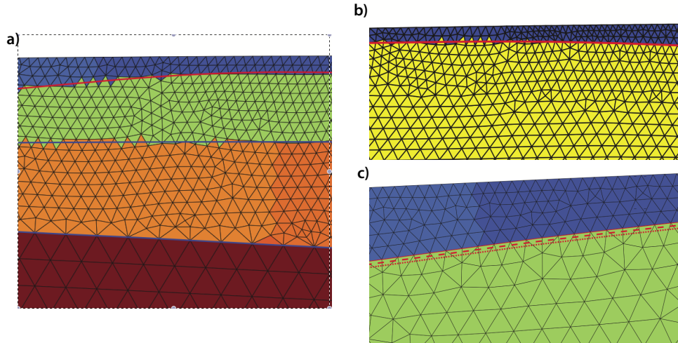
Figure 4.4: (a) Zoom of the Sharp mesh, (b) zoom of the Cutoff 2km sedi mesh and (c) zoom of the sedi200 and sedi400 mesh: the red lines are the shifted location of the sediment interface.
