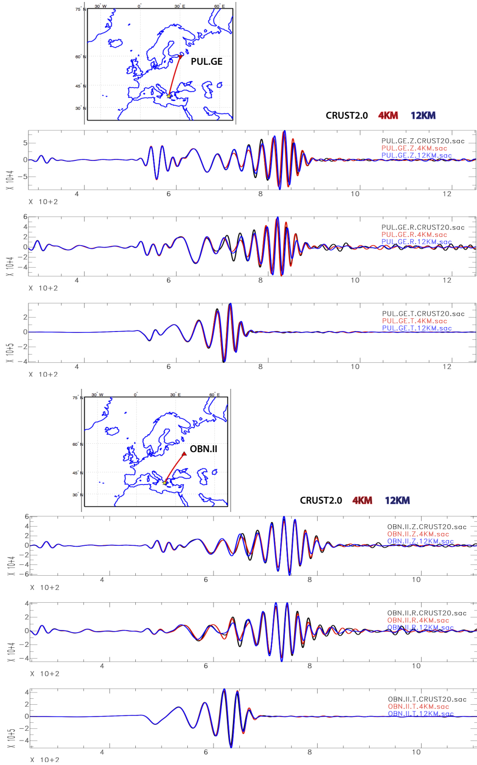
Figure 1.14: Comparison of synthetics recorded at PUL station (top), OBN station (bottom) using CRUST2.0 (black), CR-4KM (red), and CR-12KM (blue). The signals are low pass filtered with corner frequency of 0.05 Hz.
