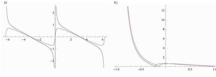
Figure B.2: Plot of the generating function of \mathbf{G} in the Haldane phase (blue line) and in the Néel phase (red line); in a) it is plotted as a function of k , while in b) we plot its absolute value as a function of z = e^{ik}
